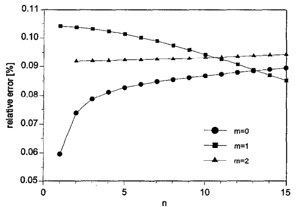
Fig. 2. Cumulated relative errors for the real and imaginary part of the g_{n, TM}^m coefficients computed by the localized approximation method and by using the integral representation given in Eq. (21). w_0 = 5 \mu\text{m} , \lambda = 0.5 \mu\text{m} , x_0 = y_0 = 2 \mu\text{m} , z_0 = 10 \mu\text{m} , m = 0, 1, 2 , n = 1, \dots, 15 .
